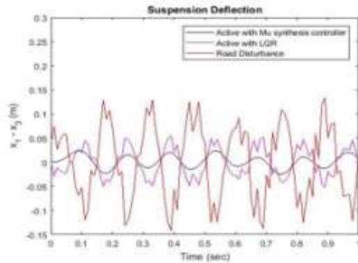
Figure 11: Suspension deflection for random road disturbance
